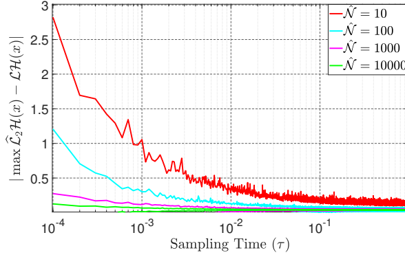
Figure 5.2: Difference between the exact analytical \mathcal{L}\mathcal{H}(x) and its approximation \hat{\mathcal{L}}_2\mathcal{H}(x) for the same initial condition x = 0.07 but different ranges of the sampling time. Plots are in the logarithmic scale in horizontal axis. The computation of \hat{\mathcal{L}}_2\mathcal{H}(x) is repeated 500 times with different numbers of data and only the maximum of \hat{\mathcal{L}}_2\mathcal{H}(x) is plotted.
