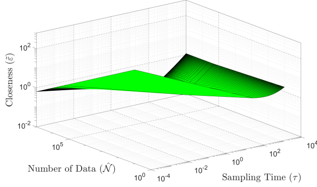
Figure 5.1: Closeness \tilde{\varepsilon} based on different ranges of the sampling time \tau and number of data \hat{N} . Plot is in the logarithmic scale.
