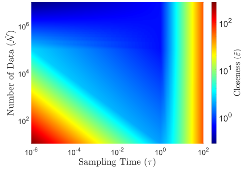
Figure 5.3: Closeness \tilde{\varepsilon} , represented by ‘colour bar’, based on different ranges of the sampling time \tau and number of data \hat{\mathcal{N}} . As it can be observed, for a fixed number of \hat{\mathcal{N}} , the total error \tilde{\varepsilon} first decreases for \tau \in [10^{-6}, 10^0] and again increases for \tau \in [10^0, 10^2] .
